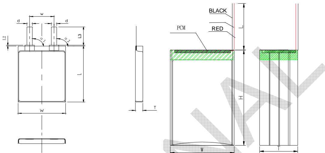
Fig.1 Dimensional Drawing of CP8543125H
