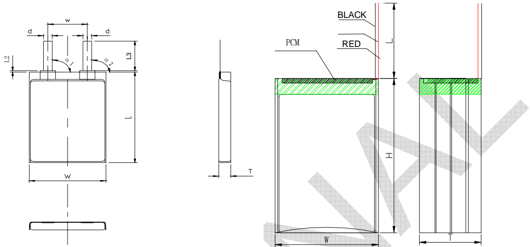
Fig.1 Dimensional Drawing of CP904560H
