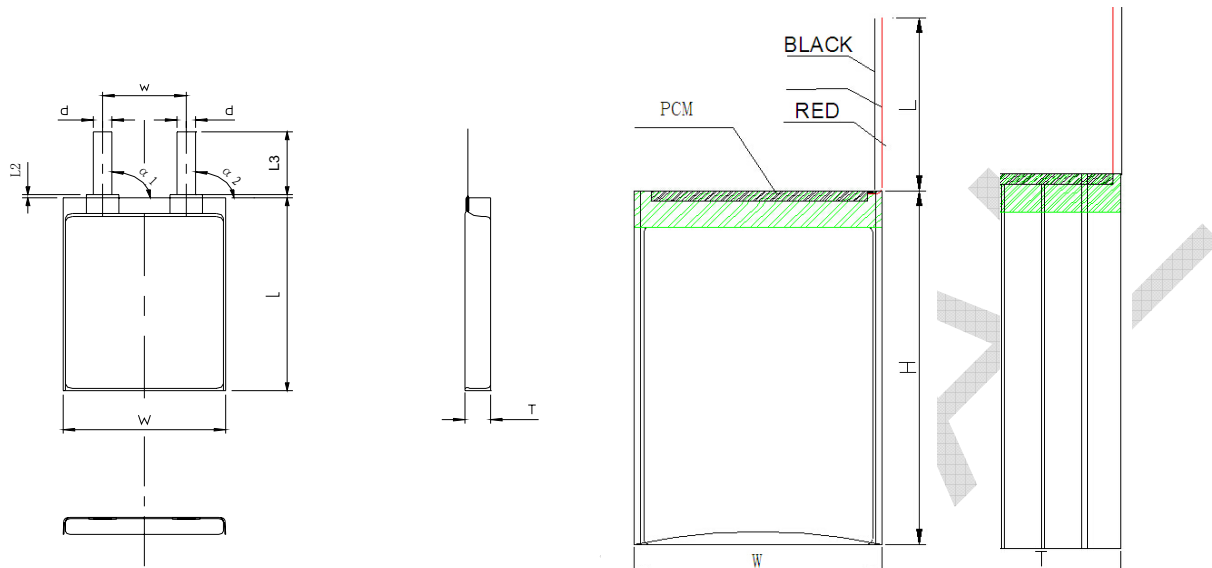
Fig.1 Dimensional Drawing of CP604893H
